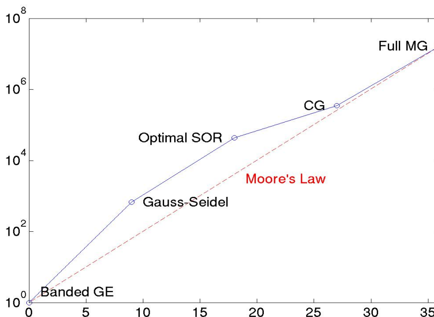
Fig. 4 Relative speed-up versus number of years: Algorithmic improvement for iterative solution methods for linear systems compared to hardware improvements. Source: Scales report, Vol. 1, Chapter 5 Enabling mathematics and computer science tools [17].
