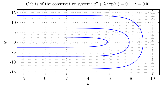
Fig. 2. Orbits corresponding to the conservative case u'' + \lambda \exp(u) = 0 .
