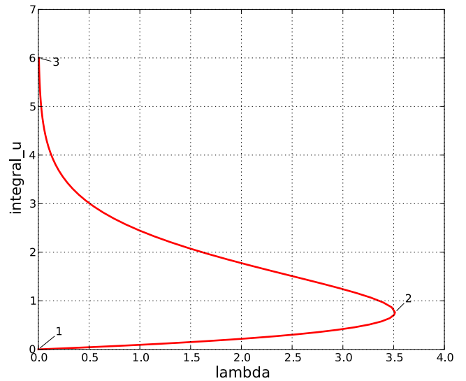
Fig. 5. The bifurcation diagram for \mu = 0 ; label 2 indicates a fold.
