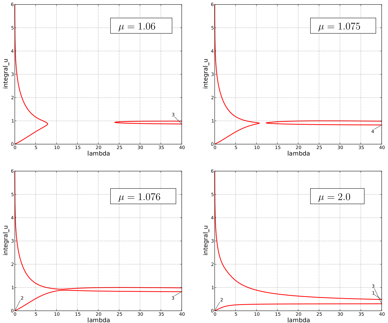
Fig. 6. One-parameter bifurcation diagrams for different values of \mu .
