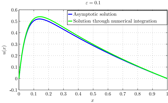
Fig. 1. Numerical and first-order asymptotic approximations of the two-point boundary problem with f(u) = \exp(u) in Eq. (1).
