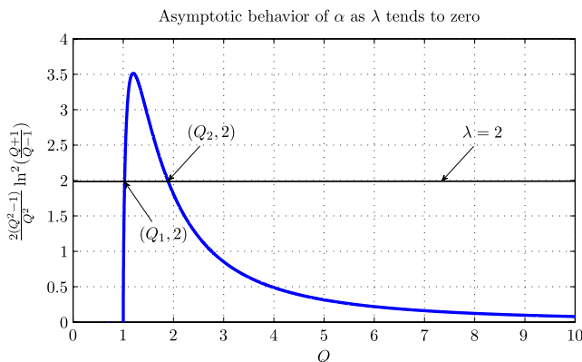
Fig. 3. Asymptotic behavior of the roots of (13) as \lambda \rightarrow 0 .
