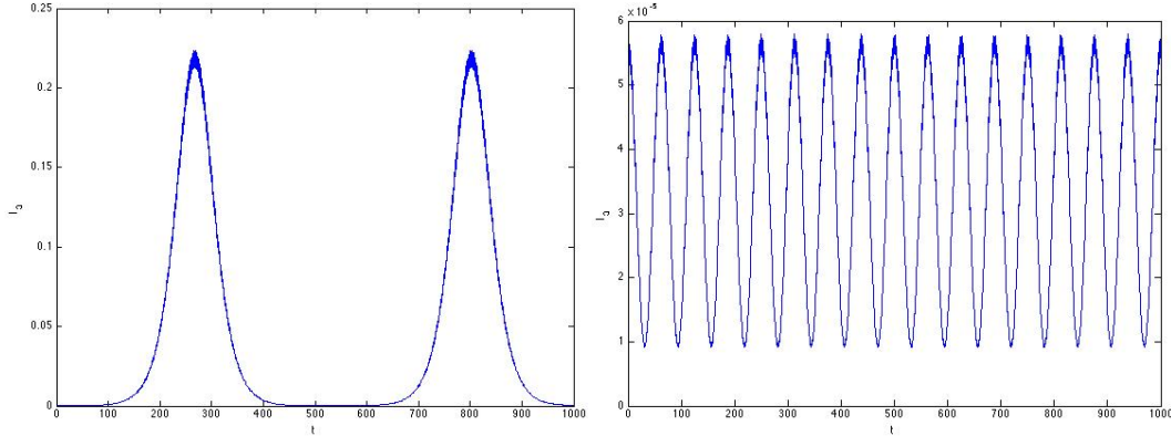
Figure 2: The action I_3 = \frac{1}{2}(\dot{x}_3^2 + \omega^2 x_3^2) in two cases of system (4) with x_1(0) = 1, x_2(0) = 0.1, x_3(0) = 0.01 , velocities zero; \varepsilon = 0.1 and 1000 time-steps. Left the case \omega^2 = 1.1 leading to instability of the x_1 normal mode, 0 < I_3 < 0.23 . Right the slightly more detuned case \omega^2 = 1.15 leading to stability of the x_1 normal mode, the fluctuations of I_3 are of size 10^{-4} .
