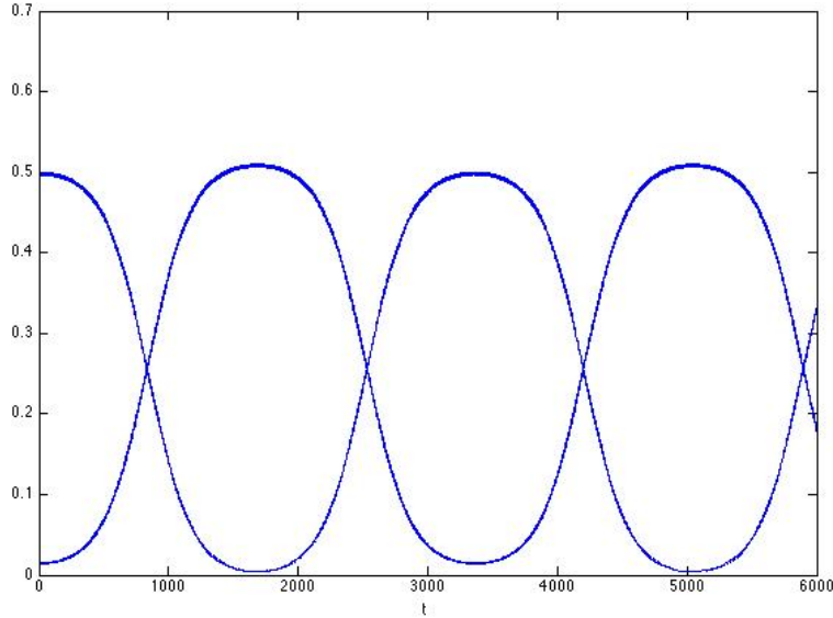
Figure 1: The actions of system (2) with x_1(0) = 1, x_2(0) = x_3(0) = 0.1 , velocities zero; \varepsilon = 0.1 and 6000 time-steps. The action I_1 = \frac{1}{2}(\dot{x}_1^2 + x_1^2) associated with the x_1 normal mode starts in 0.5 and shows recurrence on around 3400 time-steps. The sum of the actions I_2 + I_3 associated with the x_2, x_3 modes starts near zero and shows similar recurrence.
