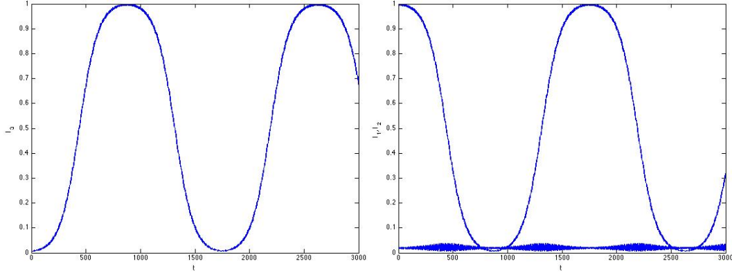
Figure 3: The actions for 3000 timesteps near the unstable x_2 normal mode of system (8) with \varepsilon = 0.1 , initial conditions x_1(0) = x_3(0) = 0.1, x_2(0) = 1 and initial velocities zero. Left the action I_3(t) = \frac{1}{2}(\dot{x}_3^2 + 2x_3^2) starting near zero and increasing to values near 1. Right I_2(t) starting at I_2(0) = 1 and I_1(t) which remains small.
