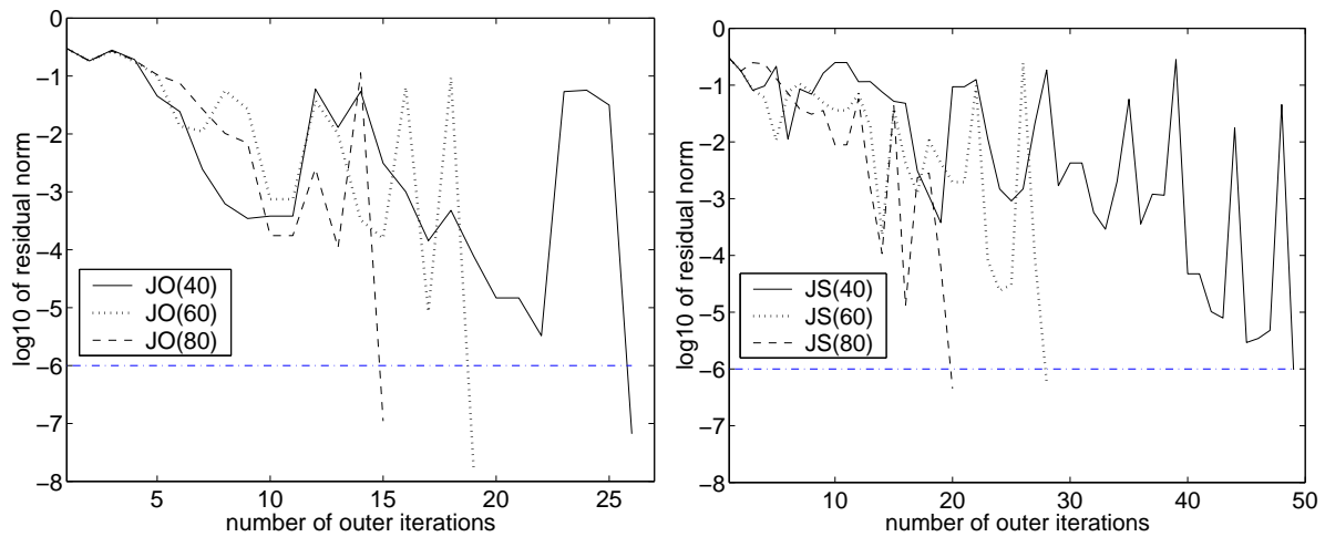
FIG. 7.3. Convergence plot for the eigenvalue closest to (0, 0) for n = 100 and u = v = [1 \ \dots \ 1]^T . The plots show the \log_{10} of the residual norm \rho_k (3.3) versus the outer iteration number k for the Jacobi–Davidson type method for the eigenvalue closest to (0, 0) using 40 (solid line), 60 (dotted line), and 80 (dashed line) GMRES steps to solve the correction equation with orthogonal projections (left plot) and skew projections (right plot), respectively.
