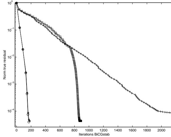
Figure 4: Norm true residual as function of the total number of iterations Bi-CGSTAB for the inexact GMRES method with fixed precision \epsilon = 10^{-6} (+), relaxed GMRES method with \epsilon = 10^{-7} (squares) and relaxed flexible GMRES preconditioned with relaxed GMRES set to a precision 0.1 (*) and the same for GMRESR in outer iteration (o).
