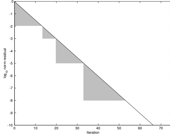
Figure 2: The grey area approximates the cost of the inner iteration when convergence in inner iteration is linear.
