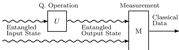
FIG. 2: Entanglement is used, \mathbb{C}^d \otimes \mathbb{C}^d model.
