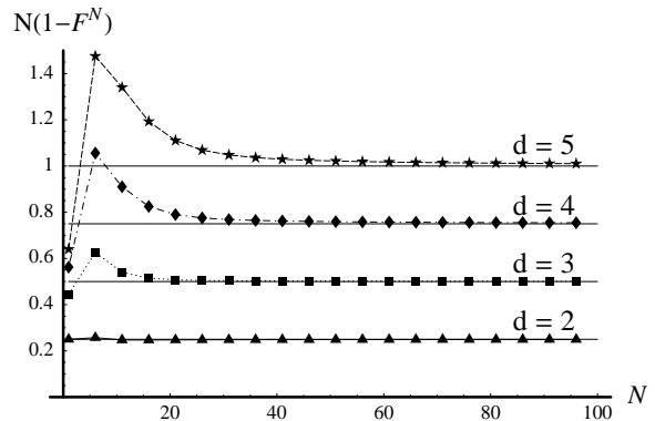
FIG. 3: The points are N(1 - F^N) as a function of N for d = 2, \dots, 5 , where F^N is the optimal fidelity obtained in Ref. [6]. The continuous lines are at the value (d-1)/4 for d = 2, \dots, 5 , (0.25, 0.5, 0.75, and 1, respectively.)
