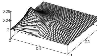
FIG. 7.6. Primal solution corresponding to Example 7.3)
