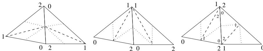
FIG. 3.2. Matching neighbours for n = 2 , and their level 1 and 2 descendants. The neighbours in the rightmost picture are not reflected neighbours, but the pair of their neighbouring children are.
